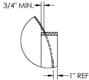
MANWAY DETAIL
